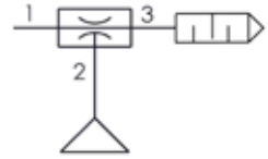
PN4029 -Vacuum ejector with pad
