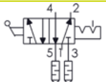
PN4067- 5/2 lever-operated valve
