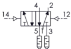
PN4024 - Air operated 5/2 double valve
