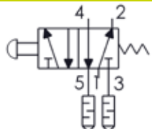
PN4110- 5/2 valve operated by mushroom push-button
