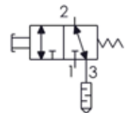
PN4018 - 3/2 NC/NO valve, operated by a push-button
