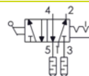
PN4021 - 5/2 valve with 2-position selector
