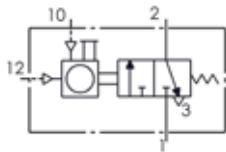
PN4012 - Pneumatic counter
