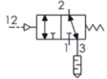
PN4020 - 3/2 NC/NO, air operated single valve
